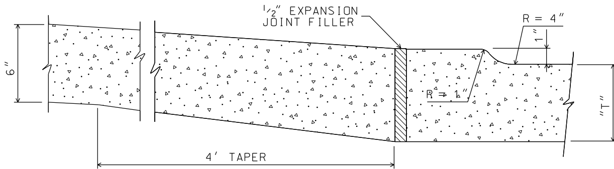
CURB DROP AT DRIVEWAY
