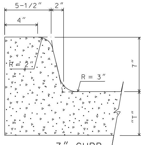
7" CURB
