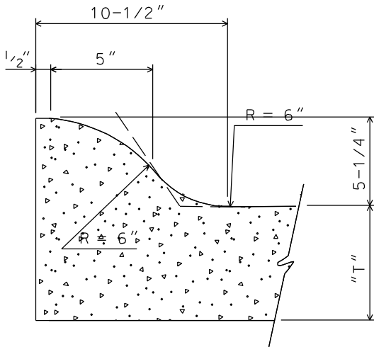
5-1/4" CURB
