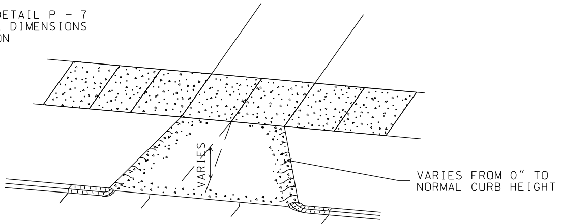
RESIDENTIAL DRIVEWAY APPROACH
