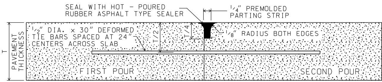
TRANSVERSE CONSTRUCTION JOINT
