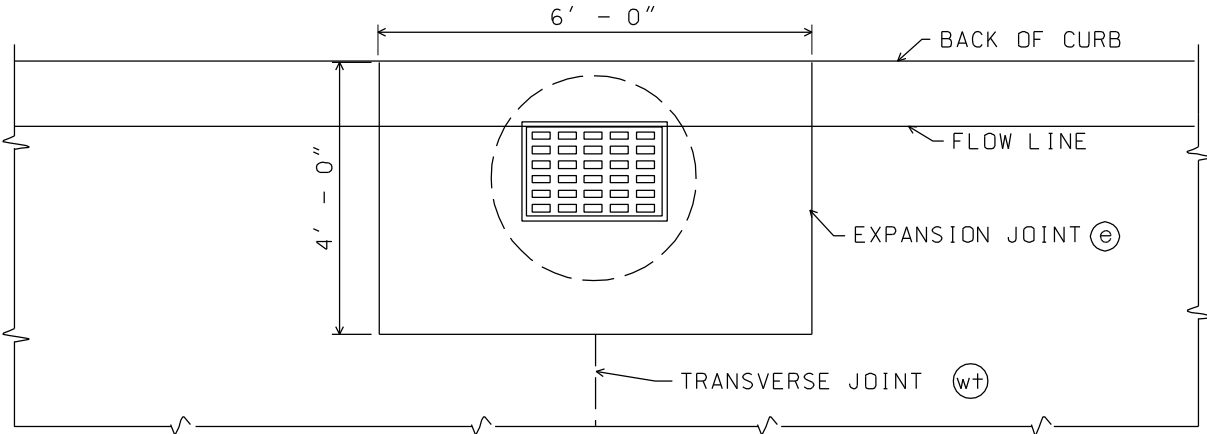
CATCH BASIN BOXOUT
