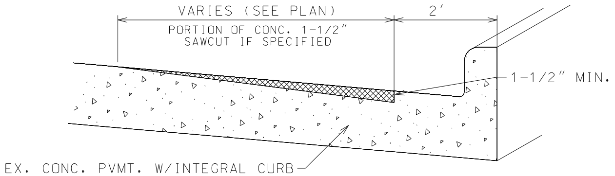
LONGITUDNAL COLD MILLING DETAIL ALONG EXIST. CONC. PVMT. W/INTERGRAL CURB
