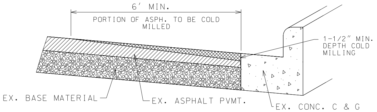
LONGITUDNAL COLD MILLING DETAIL ALONG EXIST. CONC. CURB & GUTTER
