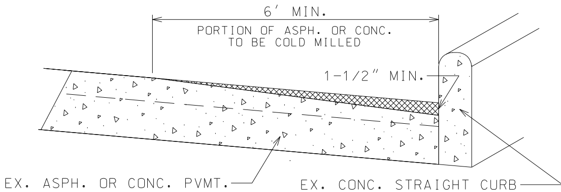
LONGITUDNAL COLD MILLING DETAIL ALONG EXIST. SEPARATE CONC. CURB
